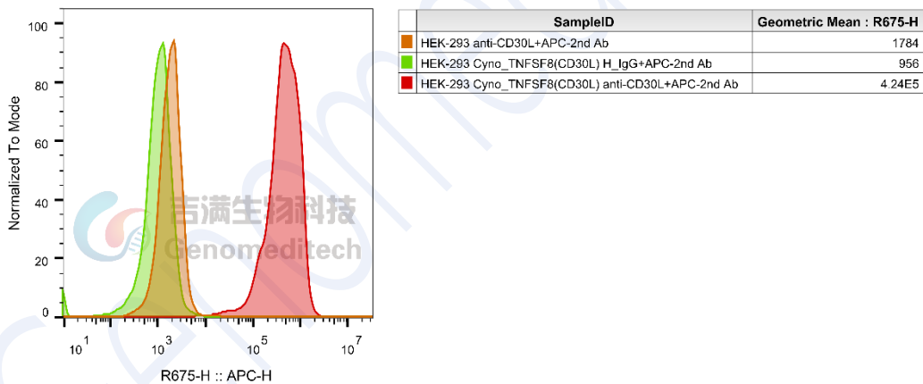
Fig. Cynomolgus_TNFSF8(CD30L) HEK-293 Cell Line (Cat. GM-C43849) was determined by flow cytometry using Anti-CD30L hIgG1 Antibody (Clone2)(Cat. GM-88399AB).
