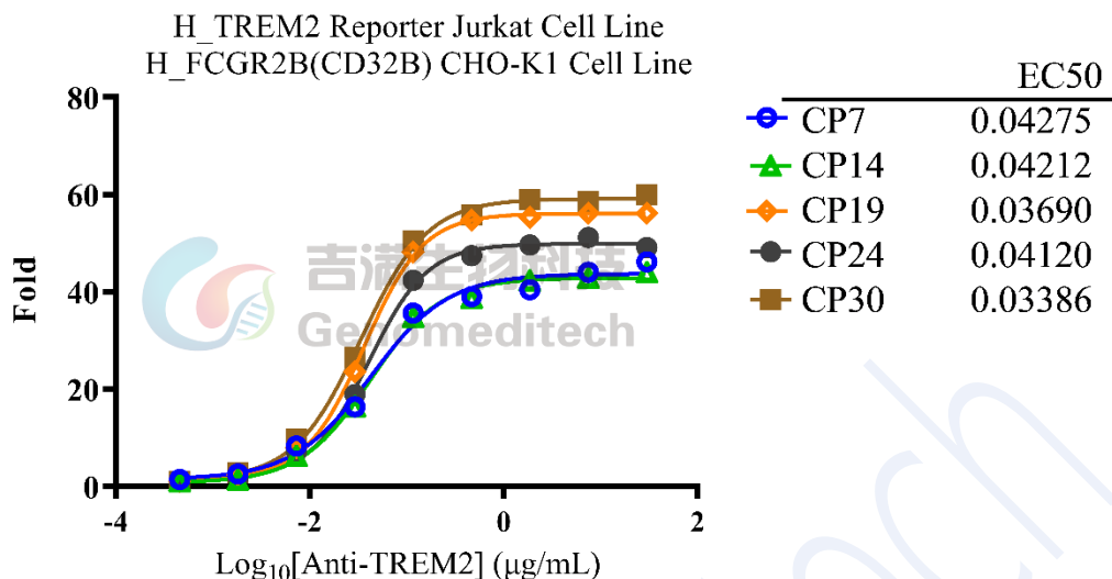
Fig 3. The passage stability of response to Research Grade Anti-Human TREM2 Antibody (al002) . The H_FCGR2B (CD32B) CHO-K1 Cell Line (Cat. GM-C16925) were seeded at a density of 1E4 cells per well in a 96-well plate and incubated overnight. The next day, serial dilutions of Research Grade Anti-Human TREM2 Antibody (al002) (antibodysystem/DHJ69201) and the passages 7, 14, 19, 24 and 30 of H_TREM2 Reporter Jurkat Cell Line (Cat. GM-C44356) at a concentration of 5E4 cells per well were added to the pre-seeded cells. The mixture was incubated for an additional 6 hours. The firefly luciferase activity was measured using the Luciferase Reporter Assay Kit (Genomeditech). Data are shown by drug mass concentration.
