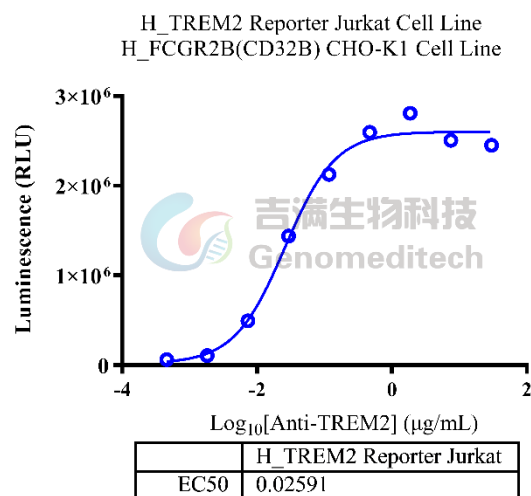
Fig 2. Response to Research Grade Anti-Human TREM2 Antibody (al002) . The H_FCGR2B (CD32B) CHO-K1 Cell Line (Cat. GM-C16925) were seeded at a density of 1E4 cells per well in a 96-well plate and incubated overnight. The next day, serial dilutions of Research Grade Anti-Human TREM2 Antibody (al002) (antibodysystem/DHJ69201) and the H_TREM2 Reporter Jurkat Cell Line (Cat. GM-C44356) at a concentration of 5E4 cells per well were added to the pre-seeded cells. The mixture was incubated for an additional 6 hours. The firefly luciferase activity was measured using the Luciferase Reporter Assay Kit (Genomeditech).The maximum induction fold was approximately [42.5]. Data are shown by drug mass concentration.
