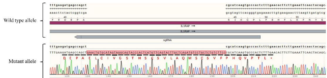
Fig 2. The Sanger sequencing of the Cynomolgus_IL1RAP HEK-293(IL1RAP KO) Cell Line showed successful knockout of Human IL1RAP.
