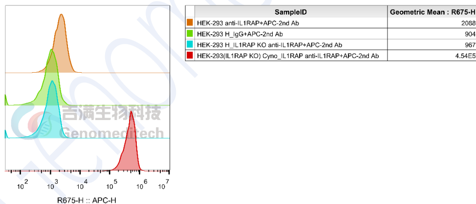
Fig 1. The Cynomolgus_IL1RAP HEK-293(IL1RAP KO) Cell Line (Cat. GM-C47998) and H_IL1RAP KO HEK-293 Cell Line (Cat. GM-C44541) were validated by flow cytometry using Anti-IL1RAP hIgG1 Antibody (48D2_VH5.GL_VL4) (Cat. GM-88388AB).
