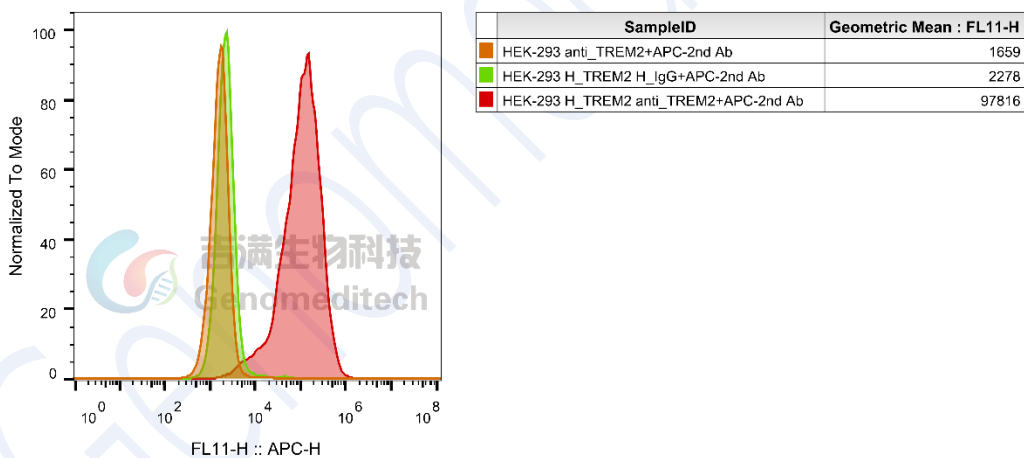
Fig 1. H_TREM2 HEK-293 Cell Line (Cat. GM-C24478) was determined by flow cytometry using Anti-H_TREM2 hIgG4 Antibody (Cat. GM-48593AB).
