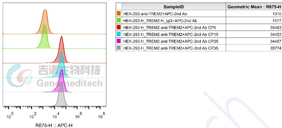
Fig 1. The passage stability of the H_TREM2 HEK-293 Cell Line (Cat. GM-C24478) was determined by flow cytometry using Anti-H_TREM2 hIgG4 Antibody (Cat. GM-48593AB).
